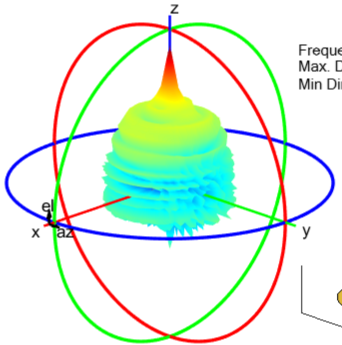
helixMultifilar
