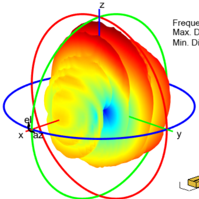
waveguideRidge
