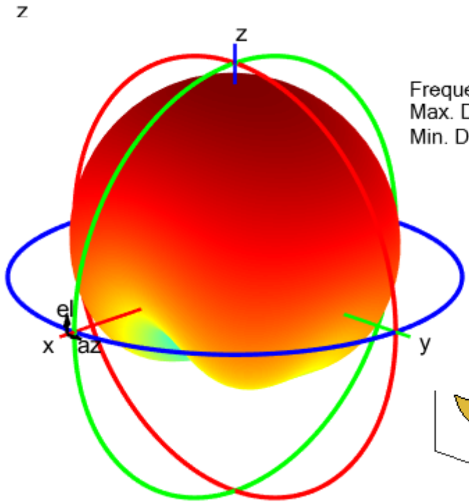
reflectorCylindrical
